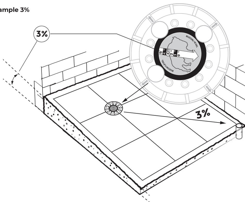
Buzon Level U-KIT-SL-80
