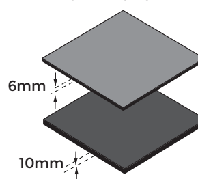
U-PAD 6-10mm
