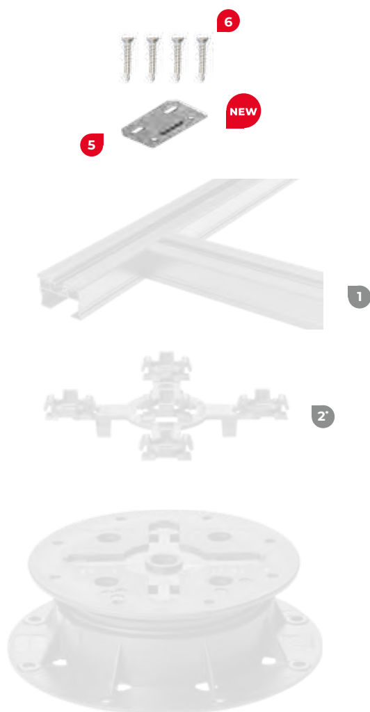
PB PEDESTAL
