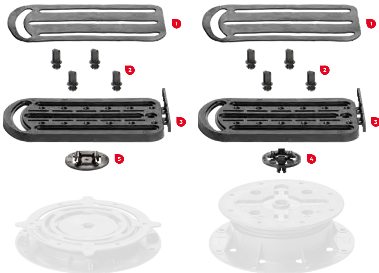
PB-0-S PEDESTAL
