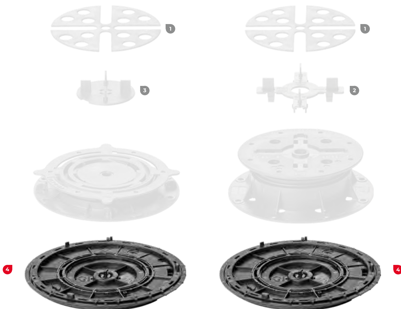
PB-0-S PEDESTAL
