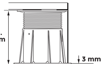
PB-4 145-245mm
