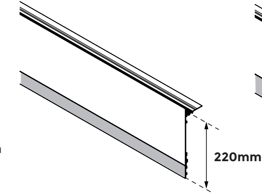
U-TFP-H180 + EXTENDER-H40
