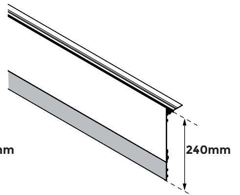
U-TFP-H180 + EXTENDER-H60
