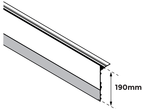
U-TFP-H130 + EXTENDER-H60
