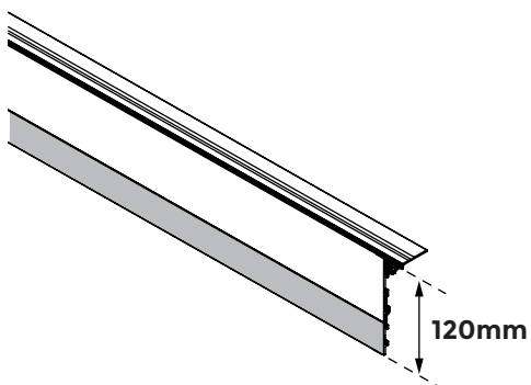
U-TFP-H80 + EXTENDER-H40
