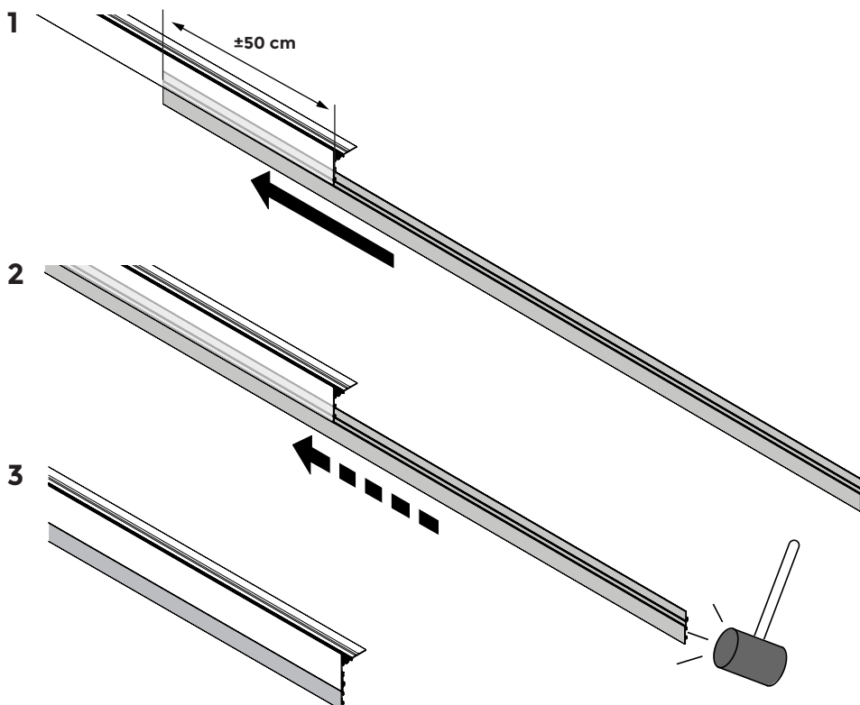
U-TFP-H80 + EXTENDER-H40
