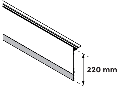
U-TFP-H180 + EXTENDER-H40
