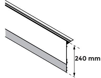
U-TFP-H180 + EXTENDER-H60
