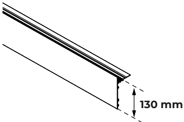
U-TFP-H130
