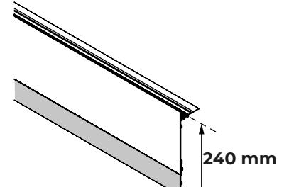
U-TFP-H180 + EXTENDER-H60
