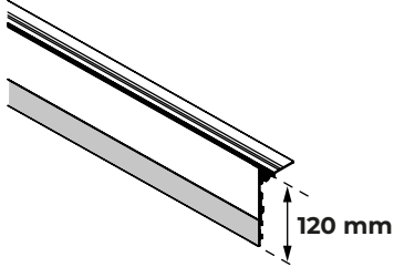
U-TFP-H80 + EXTENDER-H40
