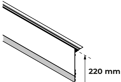
U-TFP-H180 + EXTENDER-H40
