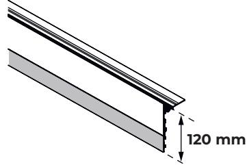
U-TFP-H80 + EXTENDER-H40
