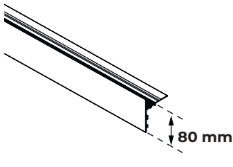
U-TFP-H80
