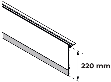
U-TFP-H180 + EXTENDER-H40
