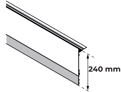
U-TFP-H180 + EXTENDER-H60
