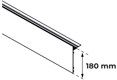
U-TFP-H180
