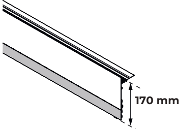
U-TFP-H130 + EXTENDER-H40
