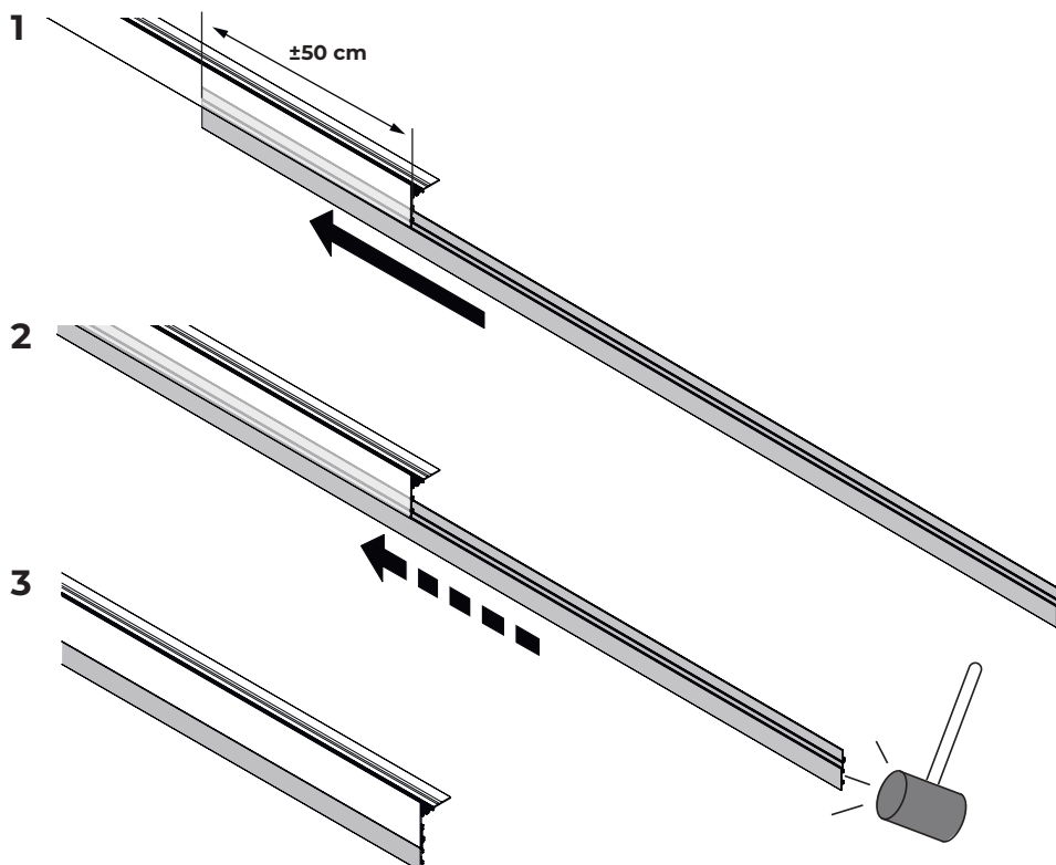
U-TFP-H80 + EXTENDER-H40
