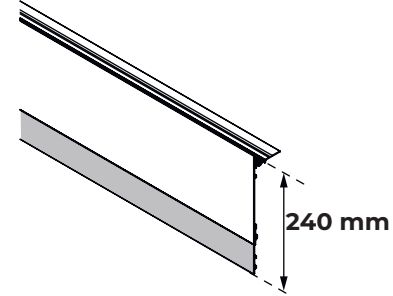
U-TFP-H180 + EXTENDER-H60
