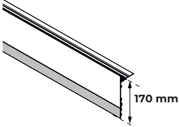
U-TFP-H130 + EXTENDER-H40
