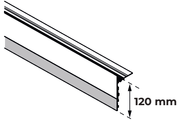
U-TFP-H80 + EXTENDER-H40
