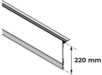
U-TFP-H180 + EXTENDER-H40
